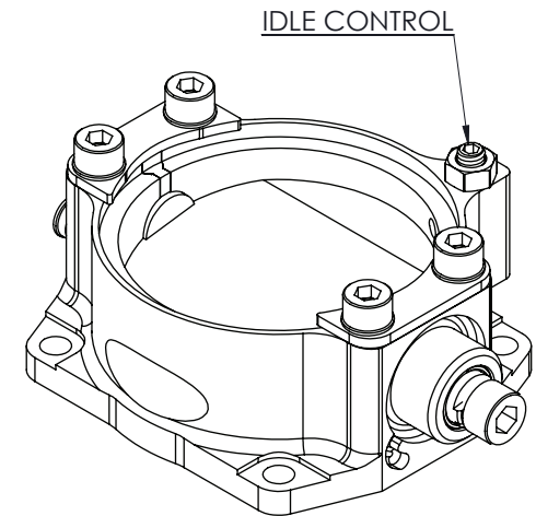
ISOMETRIC VIEW
