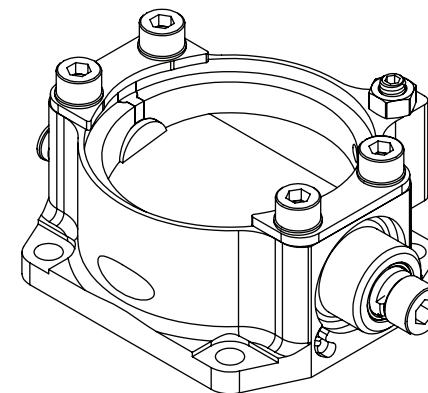
ISOMETRIC VIEW
