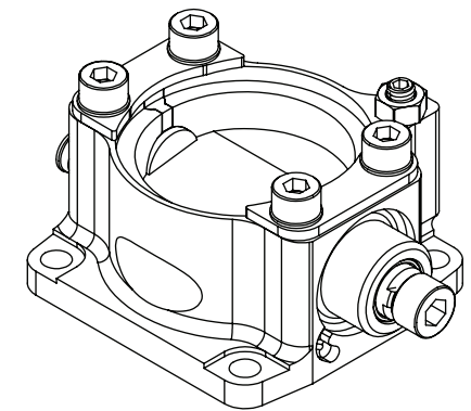
ISOMETRIC VIEW
